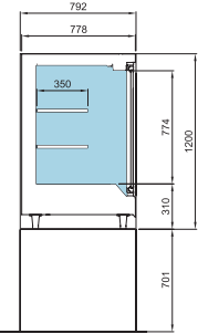
Mural de bancada Countertop mural Mural de comptoir
